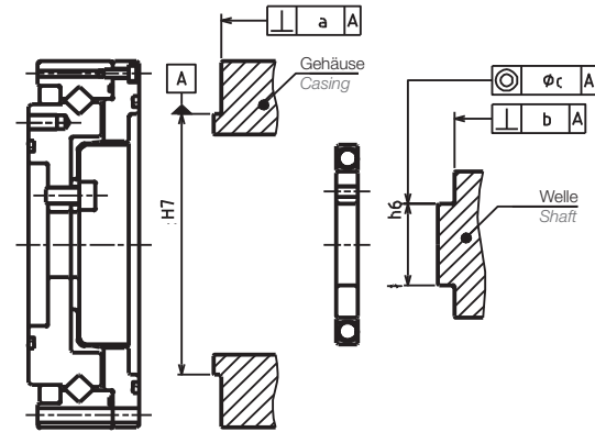
Montagetoleranzen Mounting Tolerance
