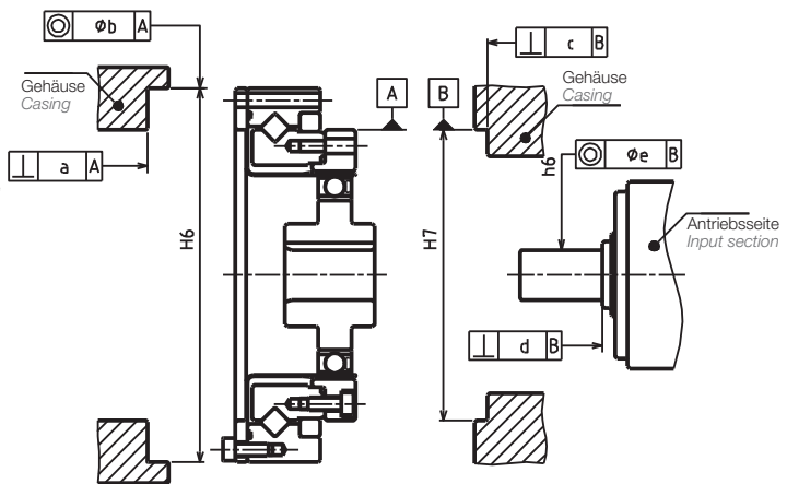
Montagetoleranz Mounting Tolerance
