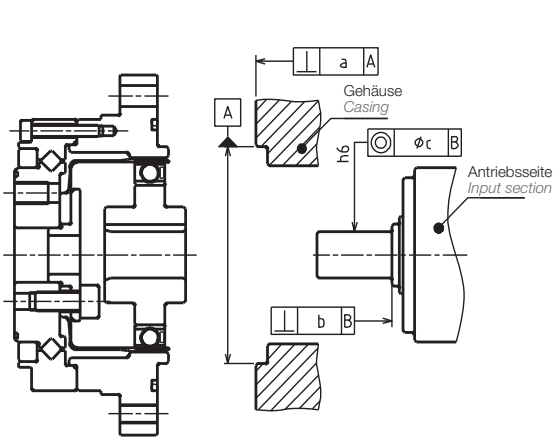
Montagetoleranz Mounting Tolerance
